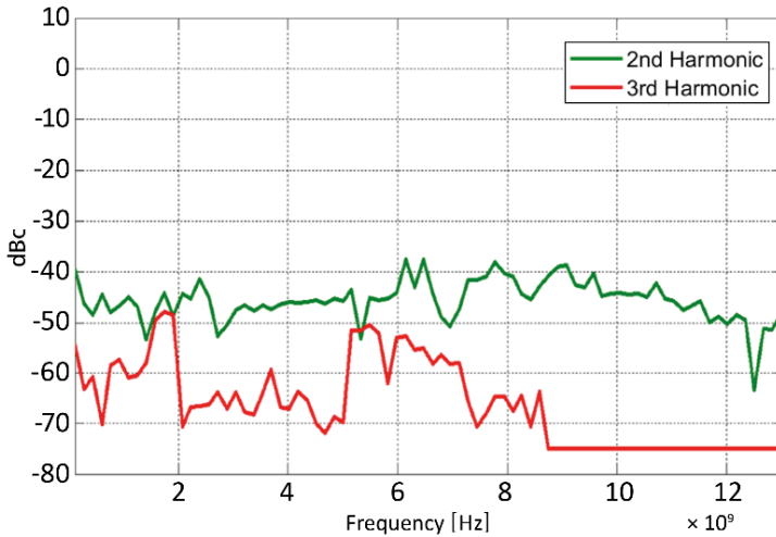
Figure 7: Harmonics Standard
