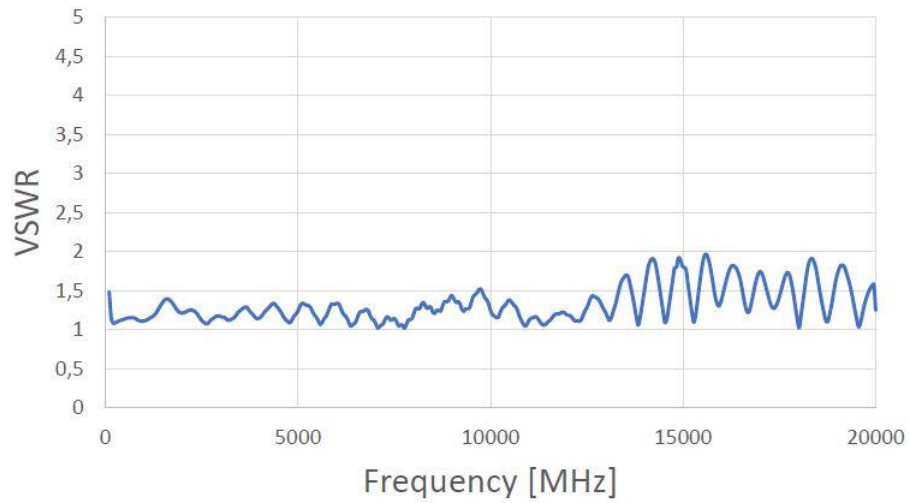
Figure 3: Typical VSWR (845-20)
